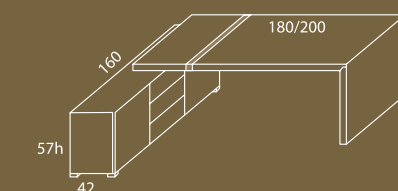
E 1218L, E 1318P E 1220L, E 1320P 190/210x170x75h
