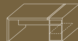
E 1118, E 1120 180/200x90x75h
